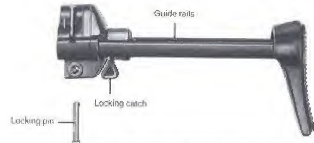
Fig. 14 Retractable butt stock
